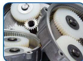
Planetary gearbox
